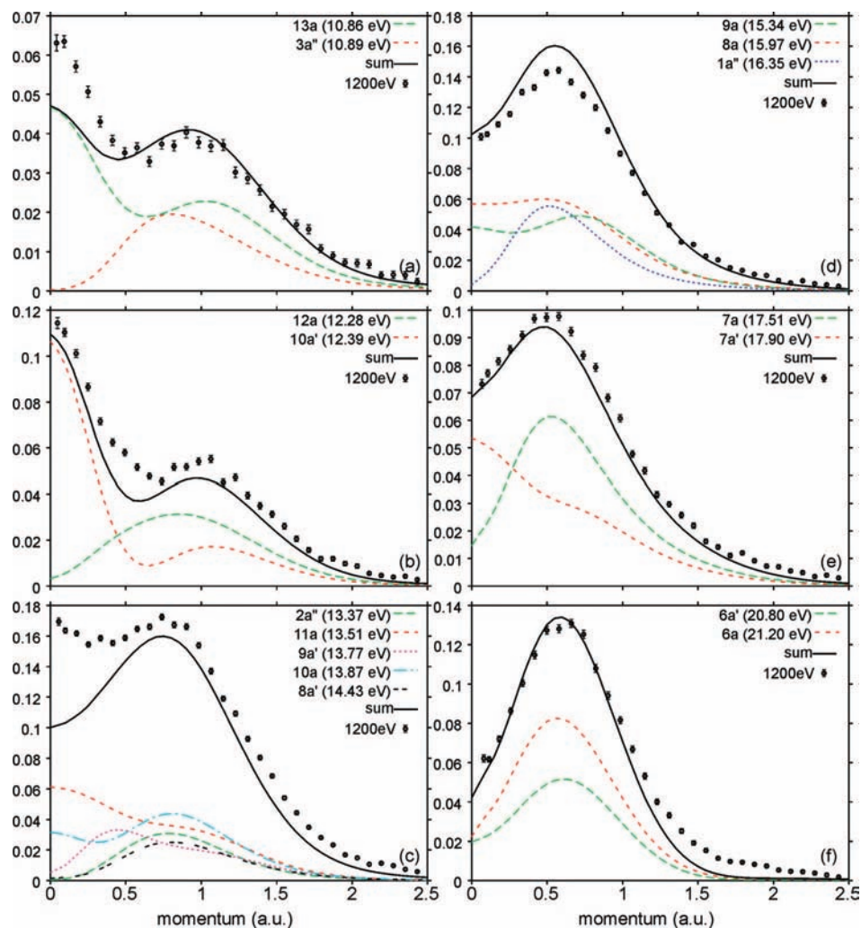
Figure 8. Decomposition of benchmark spherically and thermally averaged ADC(3)/cc-pVDZ++ electron momentum distributions ( T = 298.15 K, E_0 = 1.2 keV) into individual Dyson orbital contributions: (a) band 1 ( \epsilon_b \approx 10.9 eV), (b) band 2 ( \epsilon_b \approx 12.4 eV), (c) band 3 ( \epsilon_b \approx 13.6 eV), (d) band 4 ( \epsilon_b \approx 15.8 eV), (e) band 5 ( \epsilon_b \approx 17.8 eV), and (f) band 6 ( \epsilon_b \approx 21.0 eV).
