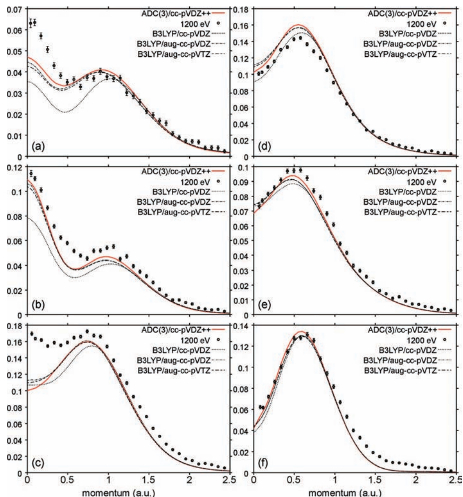
Figure 7. Spherically and thermally averaged electron momentum profiles ( T = 298.15 K) at various levels of theory as compared with experiment ( E_0 = 1.2 keV): (a) band 1 ( \epsilon_b \approx 10.9 eV), (b) band 2 ( \epsilon_b \approx 12.4 eV), (c) band 3 ( \epsilon_b \approx 13.6 eV), (d) band 4 ( \epsilon_b \approx 15.8 eV), (e) band 5 ( \epsilon_b \approx 17.8 eV), and (f) band 6 ( \epsilon_b \approx 21.0 eV).
